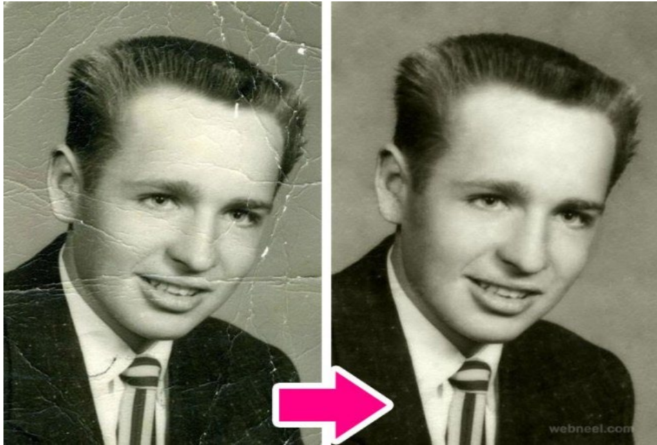
Image Restoration
